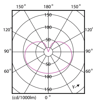
SceneSwitch LEDbulb 100W E27 A67 827-825-822 FR
