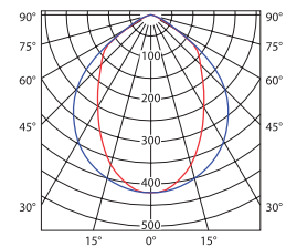
100°=420cd/1000lm [cd/1000lm] C0-C180 C90-C270 MEDIA MTH-150
