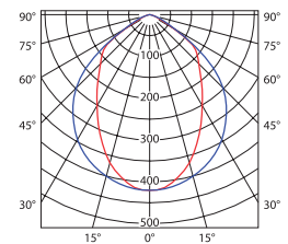
100°=420cd/1000lm [cd/1000lm] C0-C180 C90-C270 MEDIA MTH-70
