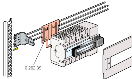
DIN rail mounting with adaptor Cat.No 0 262 39
