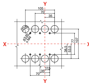
DIN rail mounting with adaptor Cat.No 0 262 39
