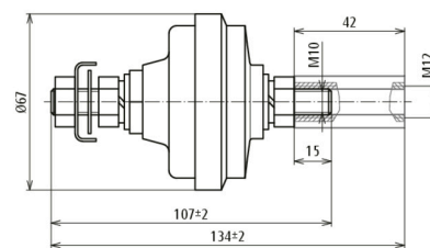
Dimension drawing DIC 10
