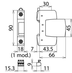
Dimension drawing DG S 320 FM
