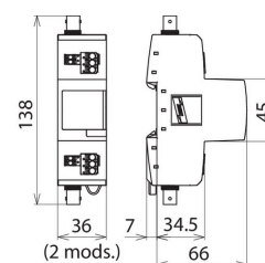
Dimension drawing DVR BNC RS485 230
