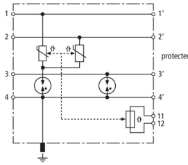
Basic circuit diagram DVR 2 BY S 150 FM
