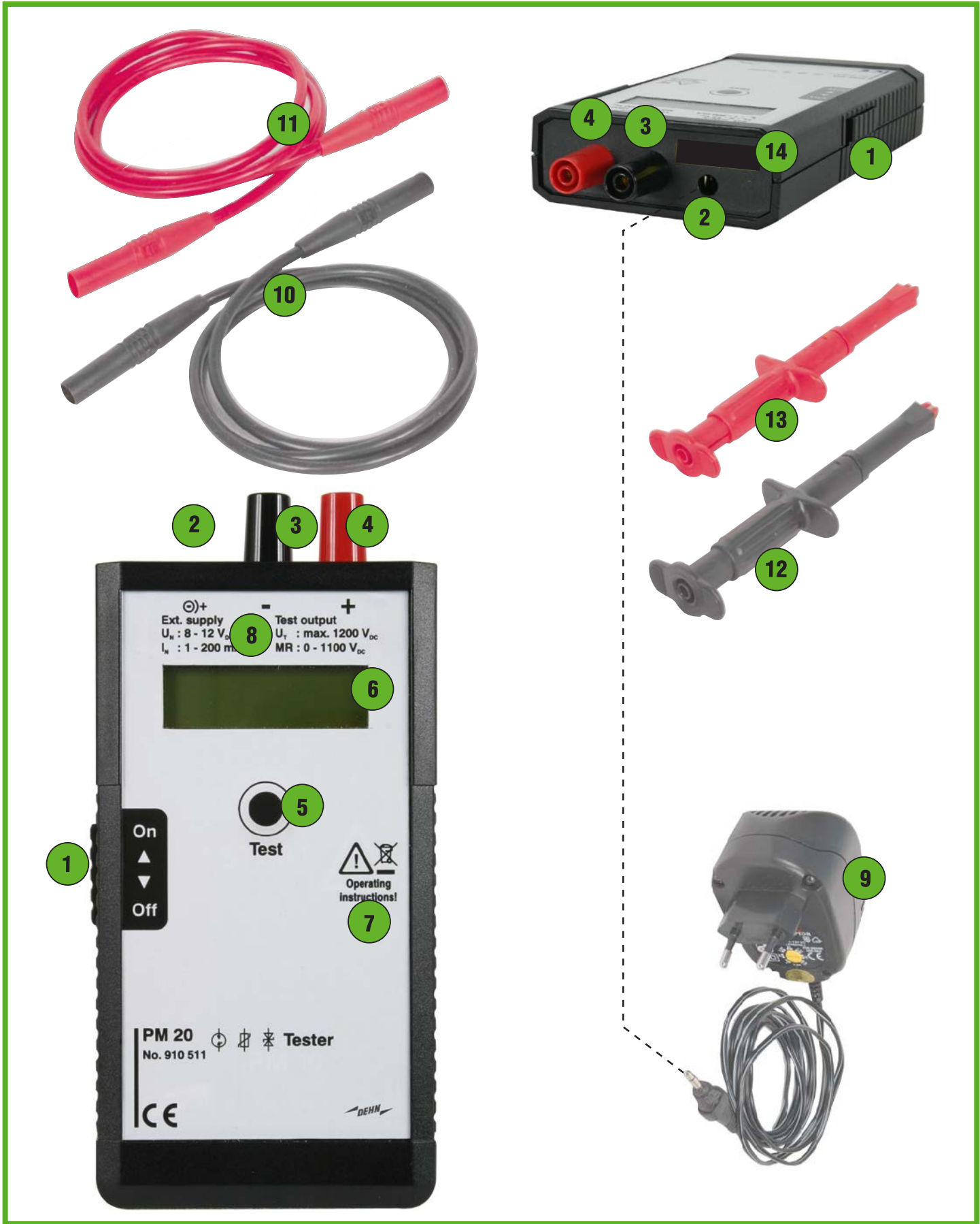
Figure 2 Device features
