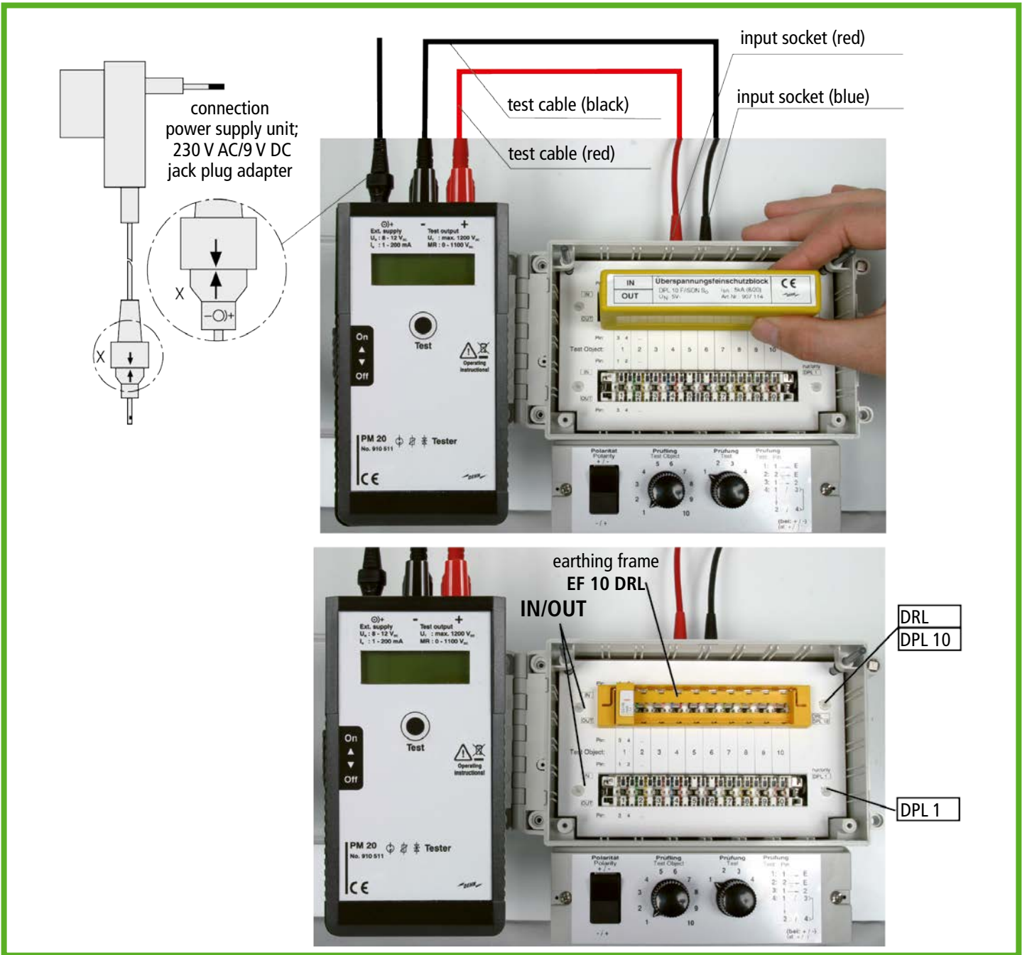
Figure 4 Test set-up 2
