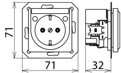
Dimension drawing NSM PRO TW
