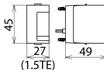
Dimension drawing DG MOD E DC 550
