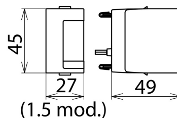
Dimension drawing DG MOD E DC 60
