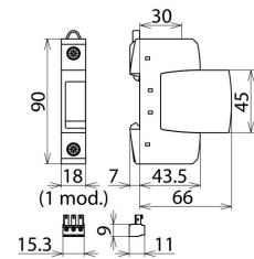
Dimension drawing DG S 385 VA FM
