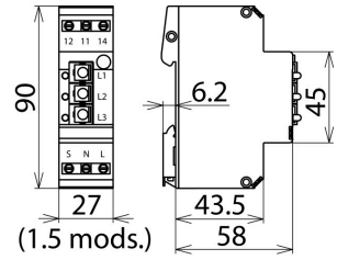
Dimension drawing DSI E 3
