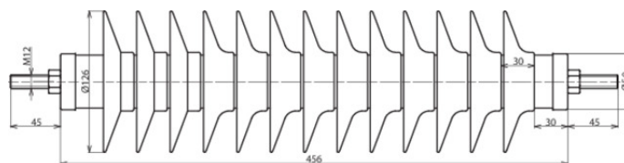
Dimension drawing DMI 51 10 1 H
