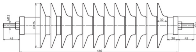
Dimension drawing DMI 48 10 1 H
