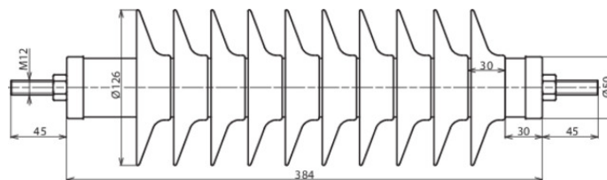
Dimension drawing DMI 39 10 1 H
