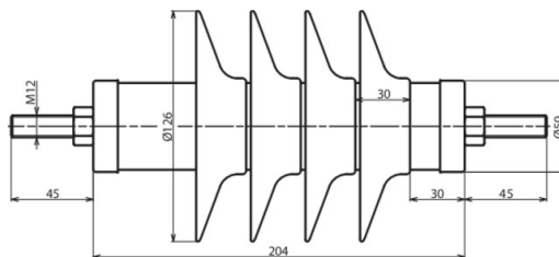
Dimension drawing DMI 21 10 1 H
