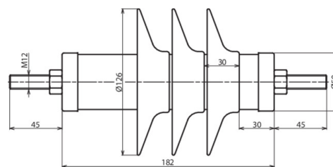
Dimension drawing DMI 18 10 1 H
