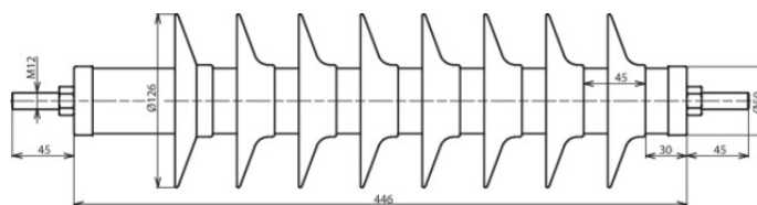
Dimension drawing DMI 48 10 1 N
