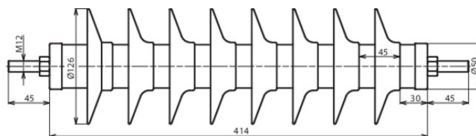
Dimension drawing DMI 45 10 1 N
