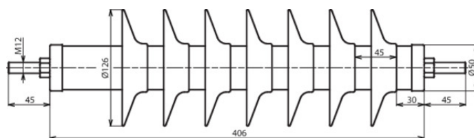
Dimension drawing DMI 42 10 1 N
