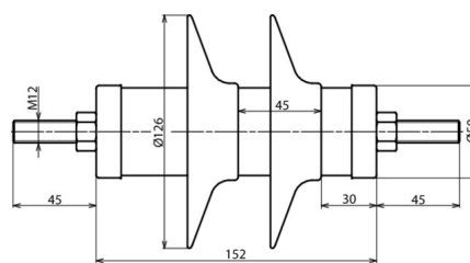
Dimension drawing DMI 12 10 1 N
