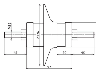
Dimension drawing DMI 3 10 1 N
