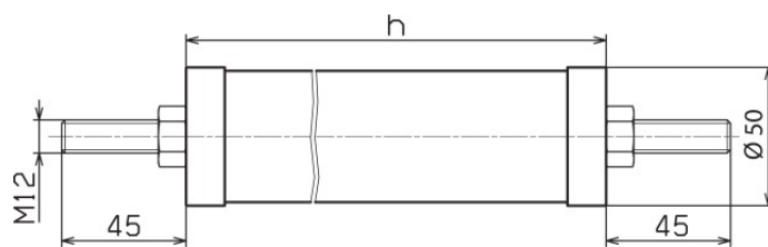
Dimension drawing DMI 45 10 1 L
