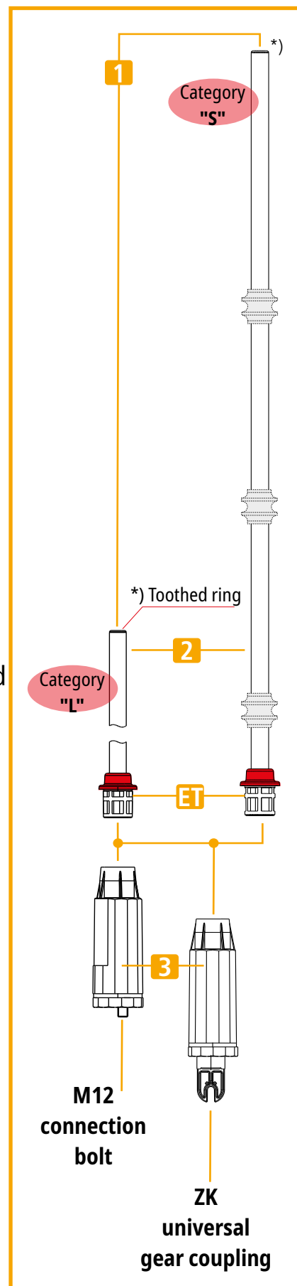
Figure 4 Structure
