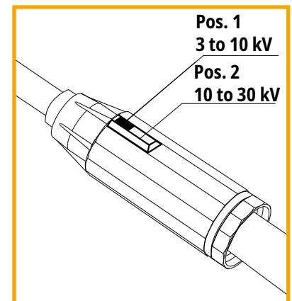
Figure 10 Nominal voltage selector switch
