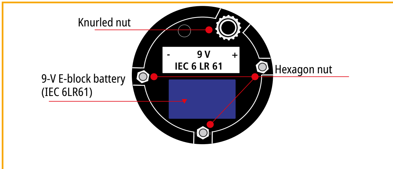
Figure 13 Underside of the electronic element
