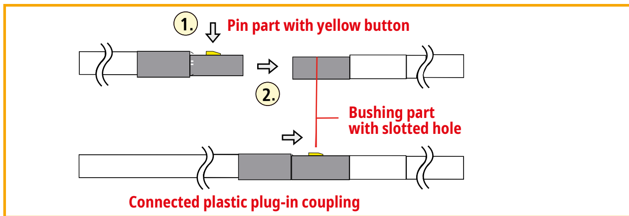
Figure 7 Plug-in coupling system
