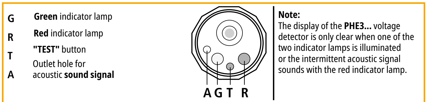
Figure 9 Indication signals
