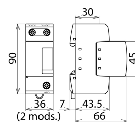
Dimension drawing DSE M 1 242
