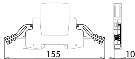
Dimension drawing SAK BXT LR
