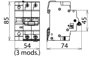
Dimension drawing POP 2 255 C32
