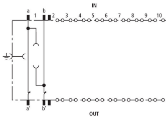
Basic circuit diagram BM 10 DRL
