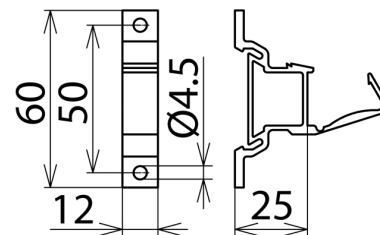
Dimension drawing SH 18X3 K
