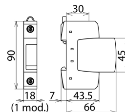
Dimension drawing DGP C S
