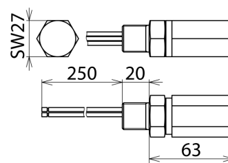
Dimension drawing DPI CD EXI+D 2X24 M
