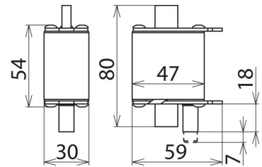
Dimension drawing VA NH00 280 FM
