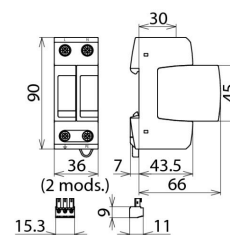
Dimension drawing DG M TT 2P 385 FM
