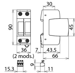
Dimension drawing DG M TT 2P 320 FM
