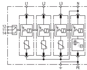
Basic circuit diagram DG M H TT 275 FM
