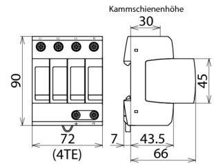
Dimension drawing DG M H TT 275
