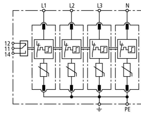
Basic circuit diagram DG M TNS 275 FM
