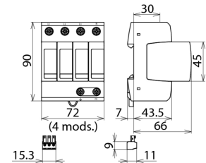
Dimension drawing DG M TNS 150 FM
