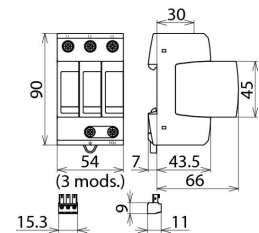
Dimension drawing DG M TNC 150 FM
