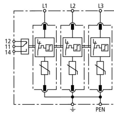
Basic circuit diagram DG M TNC 150 FM
