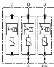
Basic circuit diagram DG M TNC 440
