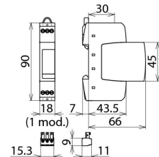
Dimension drawing DR M 2P 75 FM
