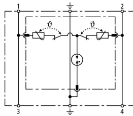
Basic circuit diagram DR M 2P 255
