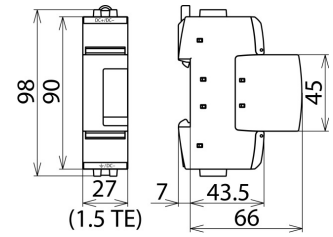
Dimension drawing DG SE DC 900
