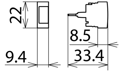
Dimension drawing DRL RD 48
