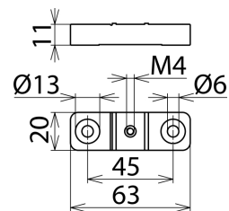
Dimension drawing ST AS SAK K
