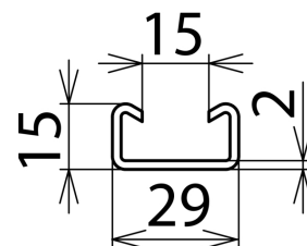
Dimension drawing AK SAK 1000 V2A
