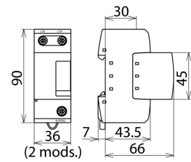
Dimension drawing DB M 1 150
