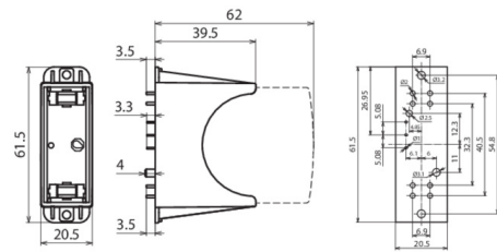
Dimension drawing DG PCB 275 FM
