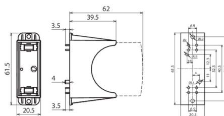
Dimension drawing DG PCB PV 30
